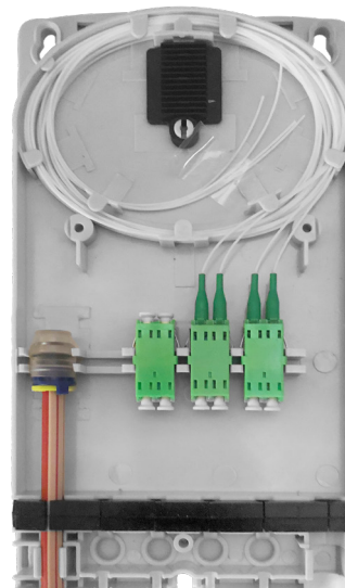
SDU-Wallbox-SP Exemplary full occupancy for supported expansion with LC/APC adapters and pigtails plus input with cable protection tube.
